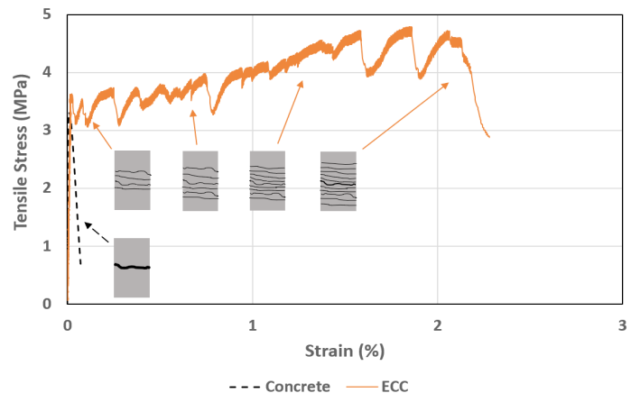
Figure 4: Tensile Properties Evaluation of Moderate Ductility ECC by Uniaxial Tensile Test.
