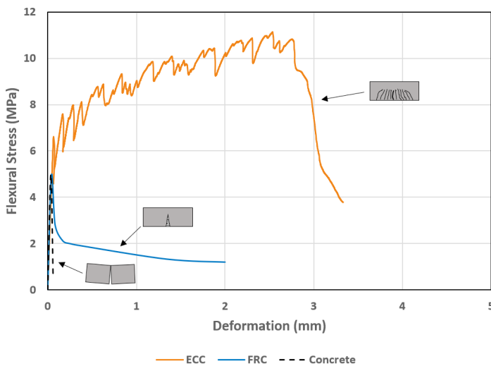
Figure 3: Flexural Performance of Moderate Ductility ECC, Fiber Reinforced Concrete (FRC) and Concrete (100 x 100 x 350 mm beams according to ASTM C1609).
