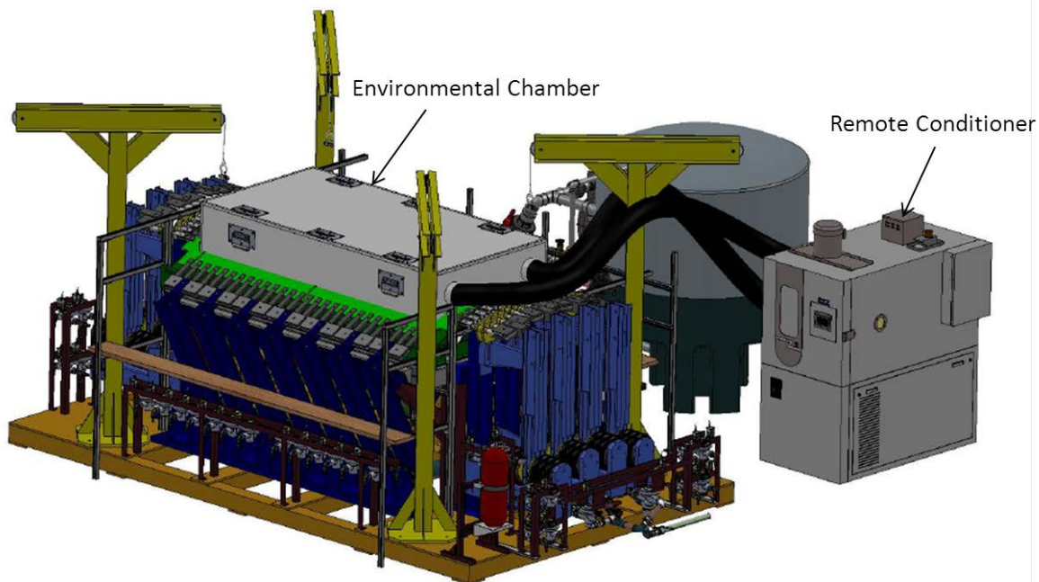
Figure 9 FAA's FASTER fixture for mechanical and environmental loading of fuselage panels.
