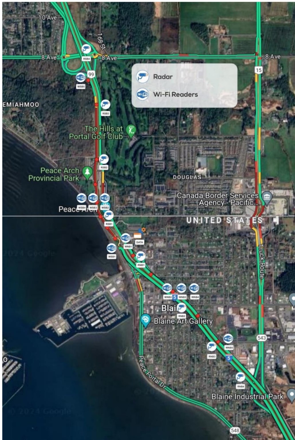
Figure 6. Proposed Roadside BWT Measurement Technologies
