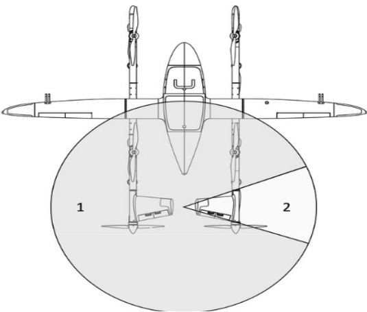
Figure 7 - AircraM Taillight Areas
