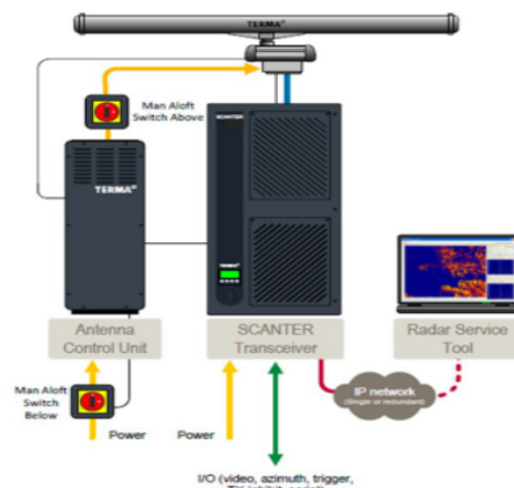
Visual Depiction of BVLOS Radar Architecture working to get information to User.
