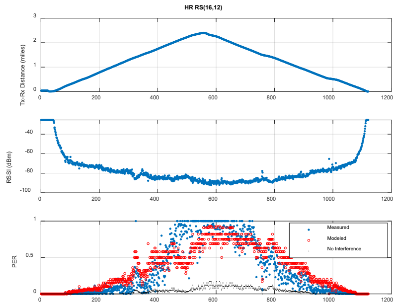
Figure 19: Performance in case of half rate with RS(16,12) coding
