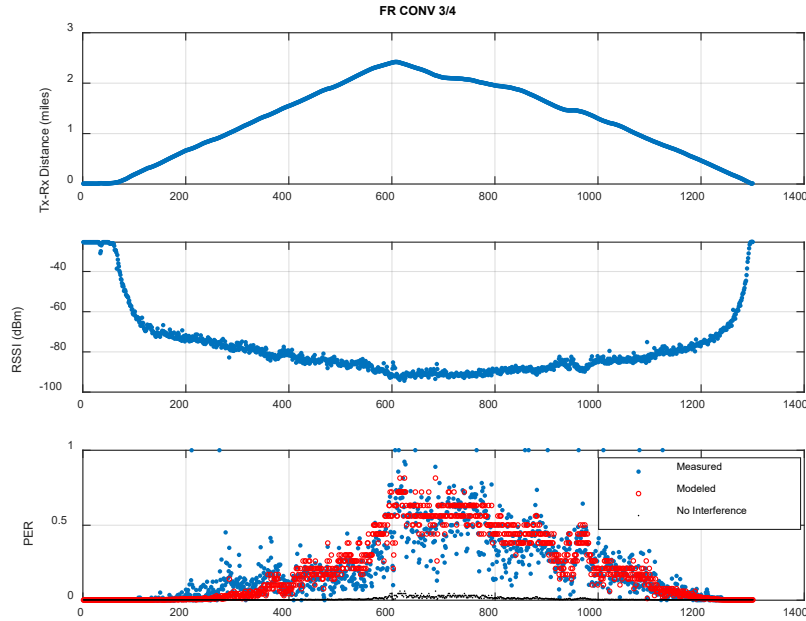
Figure 22: Performance in case of half rate with convolutional 3/4 coding
