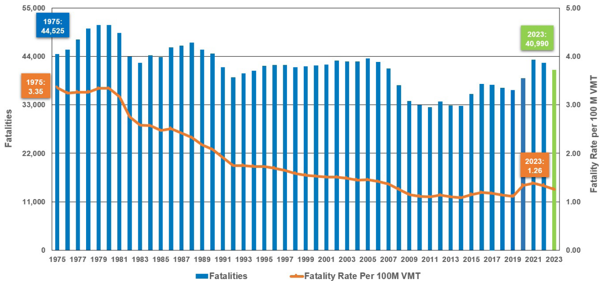
Fatalities and Fatality Rates per 100 Million Vehicle Miles Traveled, 1975-2023
